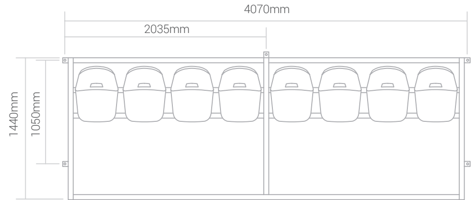
fixing tab positions for 8 person curved dugout
